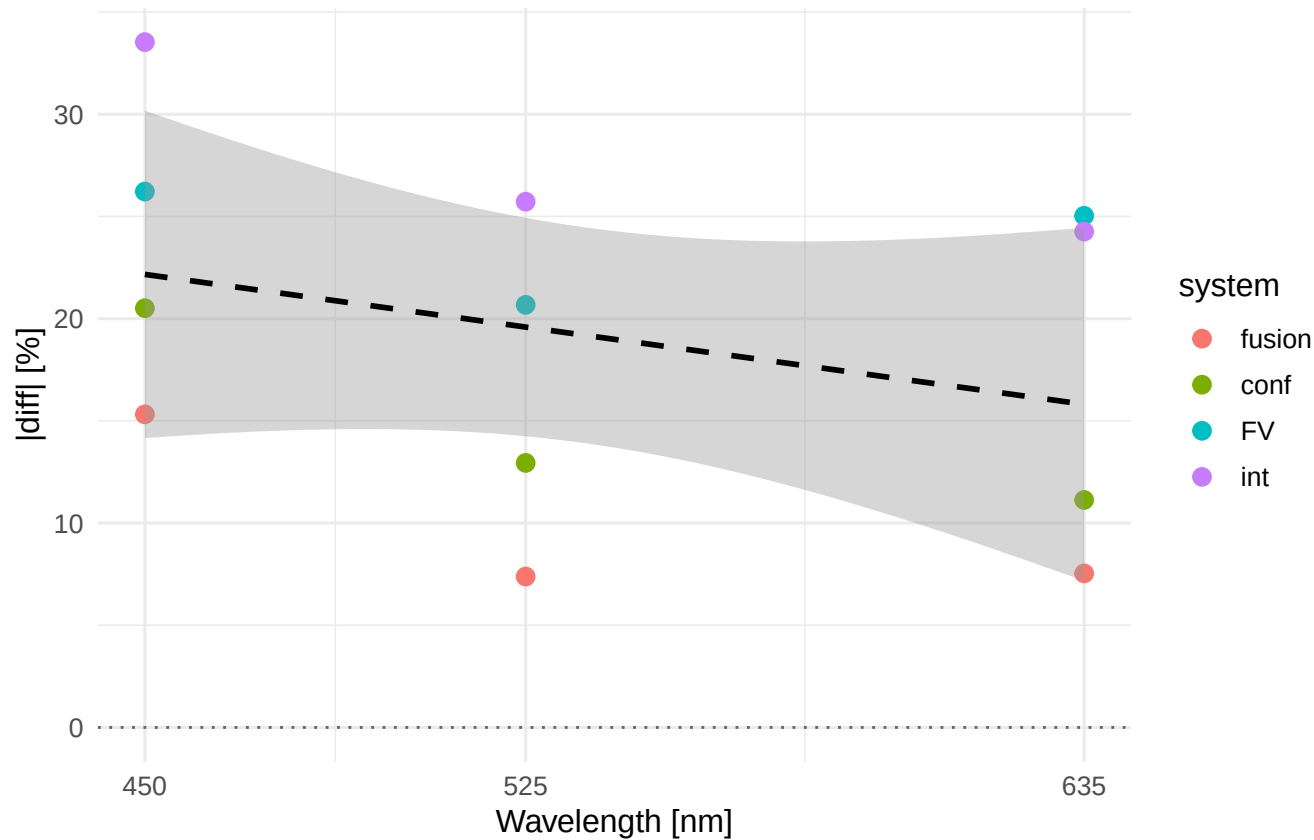
Rku |diff|% vs wavelength Material/process: MO58A_HON
