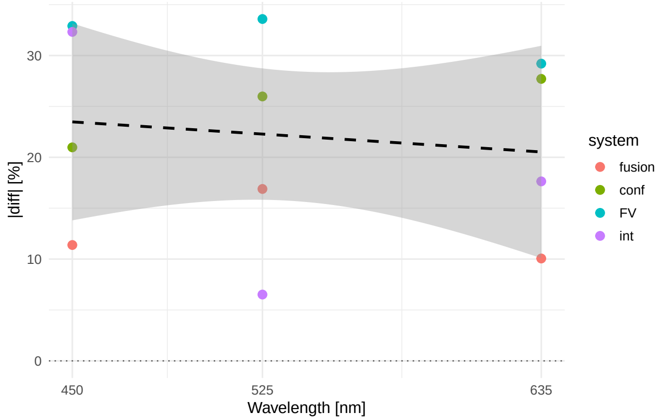
Rku |diff|% vs wavelength Material/process: Ti6Al4V_GLA
