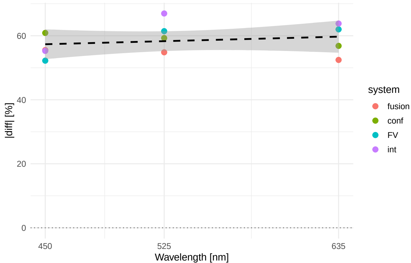
Rp |diff|% vs wavelength Material/process: Al7075_TR
