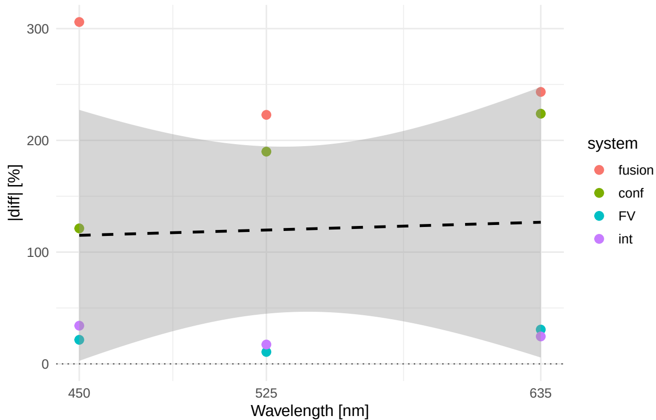
Rp |diff|% vs wavelength Material/process: C45_WEDM_F
