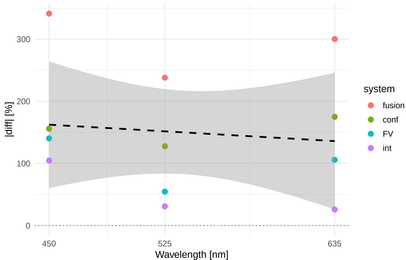
Rp |diff|% vs wavelength Material/process: ELLOR_HON
