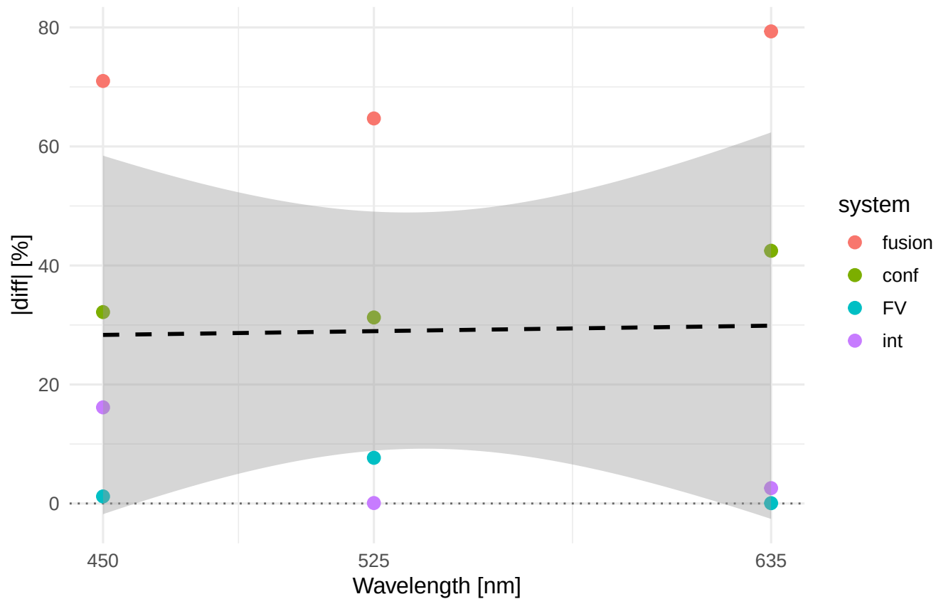
Rp |diff|% vs wavelength Material/process: ELLOR_TF
