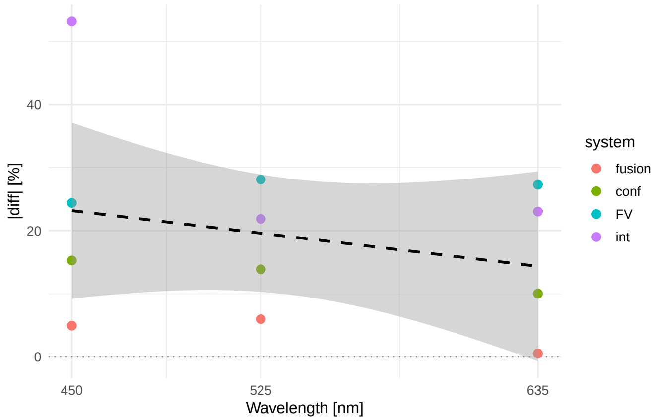
Rp |diff|% vs wavelength Material/process: ELLOR_TR
