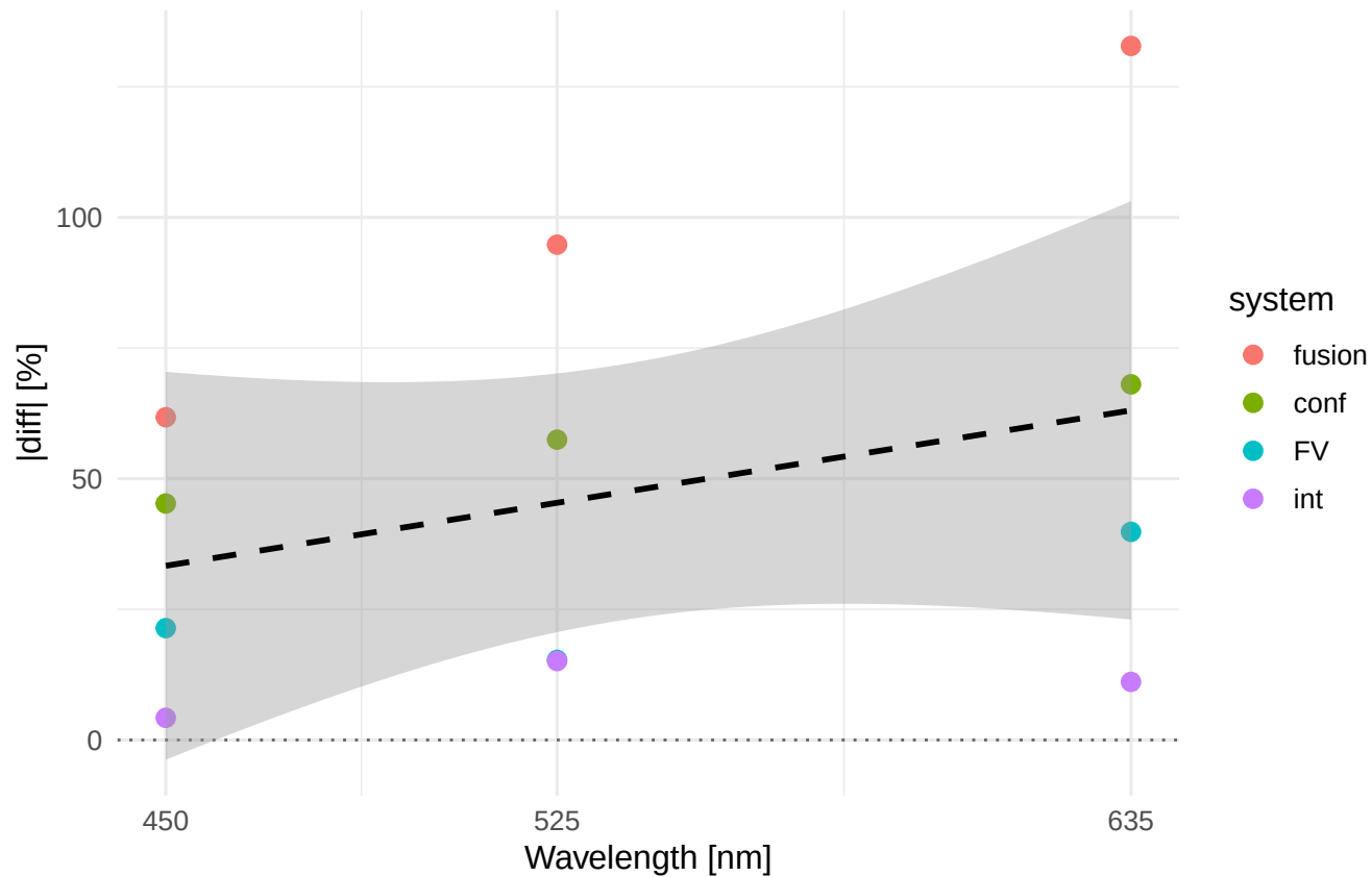
Rp |diff|% vs wavelength Material/process: MO58A_GLA
