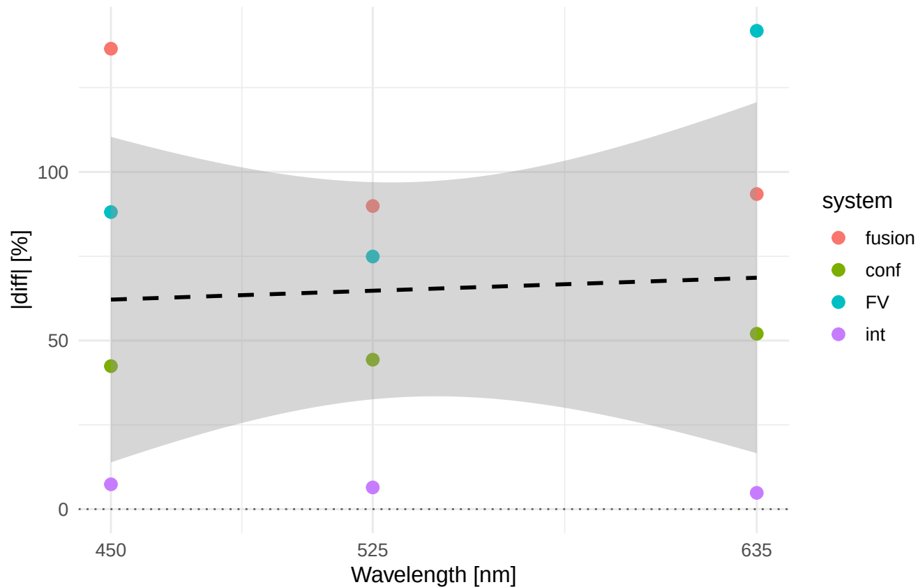
Rp |diff|% vs wavelength Material/process: MO58A_GRI
