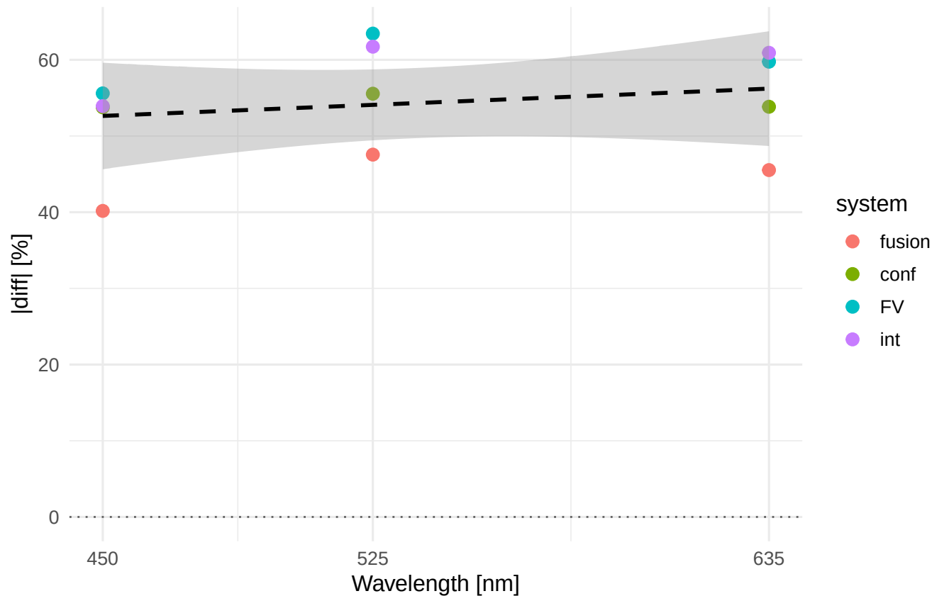
Rp |diff|% vs wavelength Material/process: MO58A_TF
