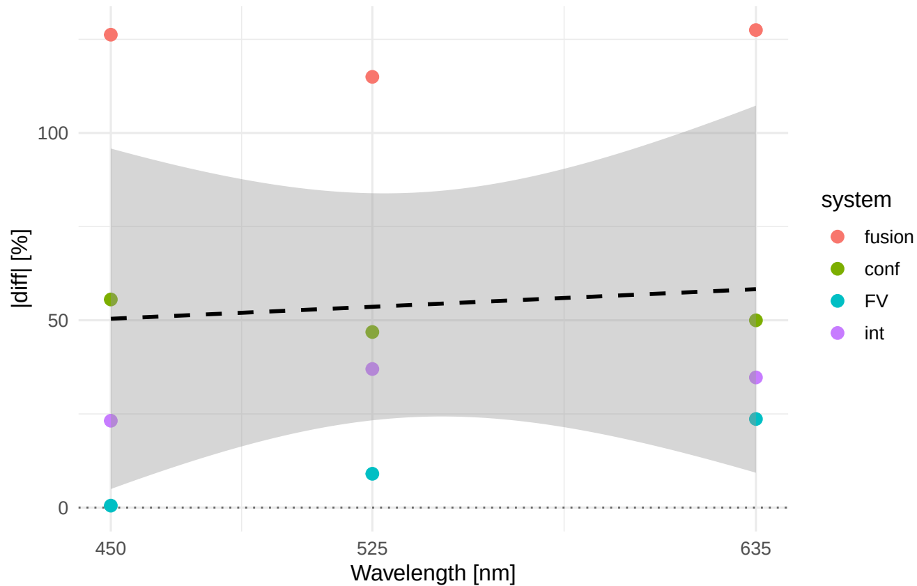
Rp |diff|% vs wavelength Material/process: Ti6Al4V_GLA
