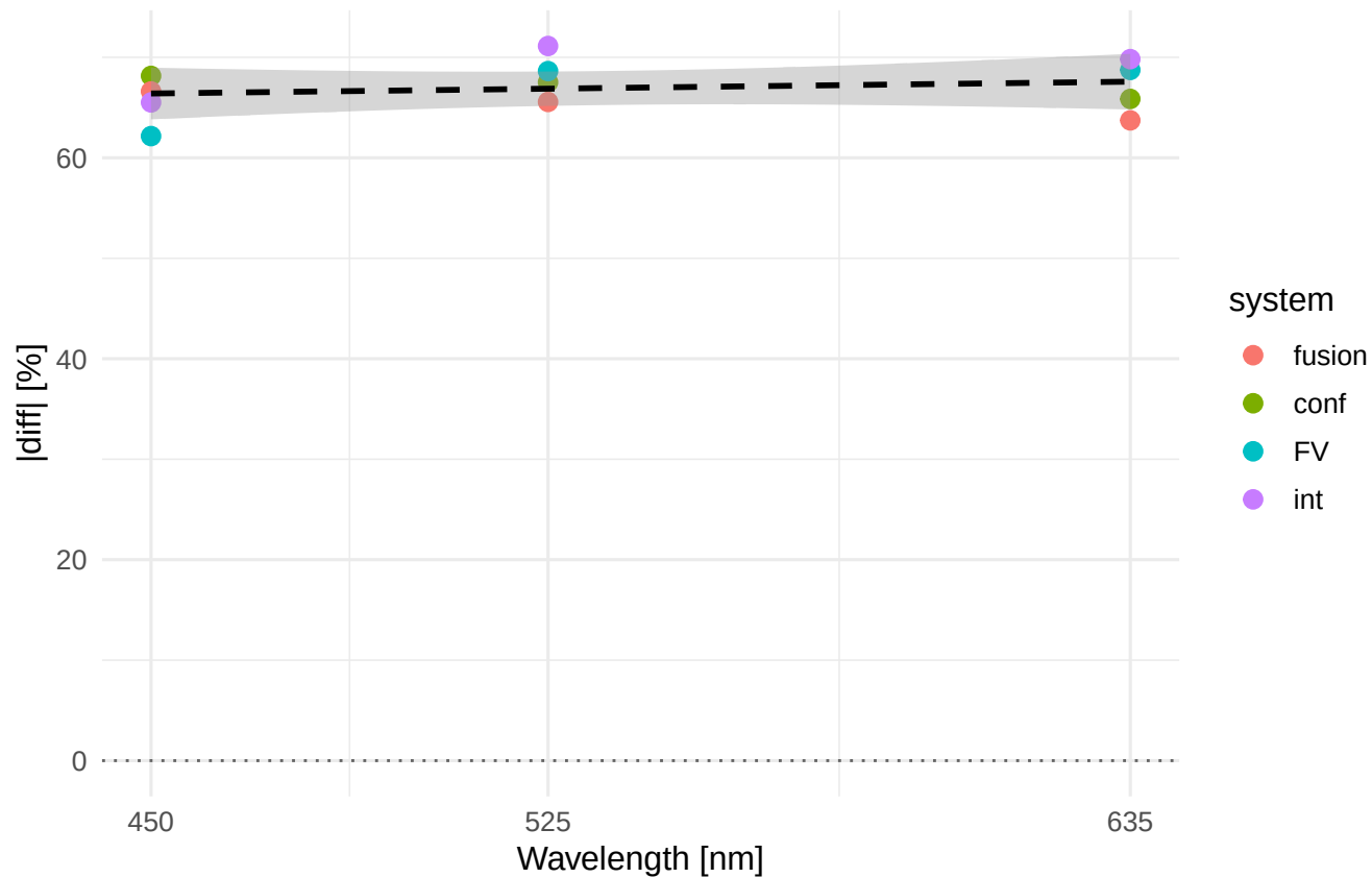
Rq |diff|% vs wavelength Material/process: Al7075_TR
