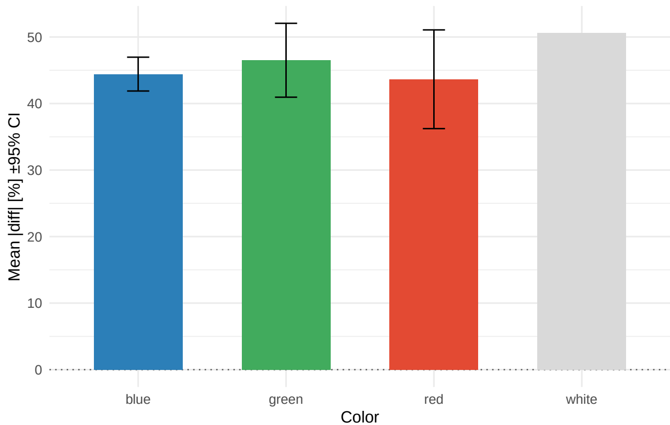
Rq effect by color Material/process: C45_MR
