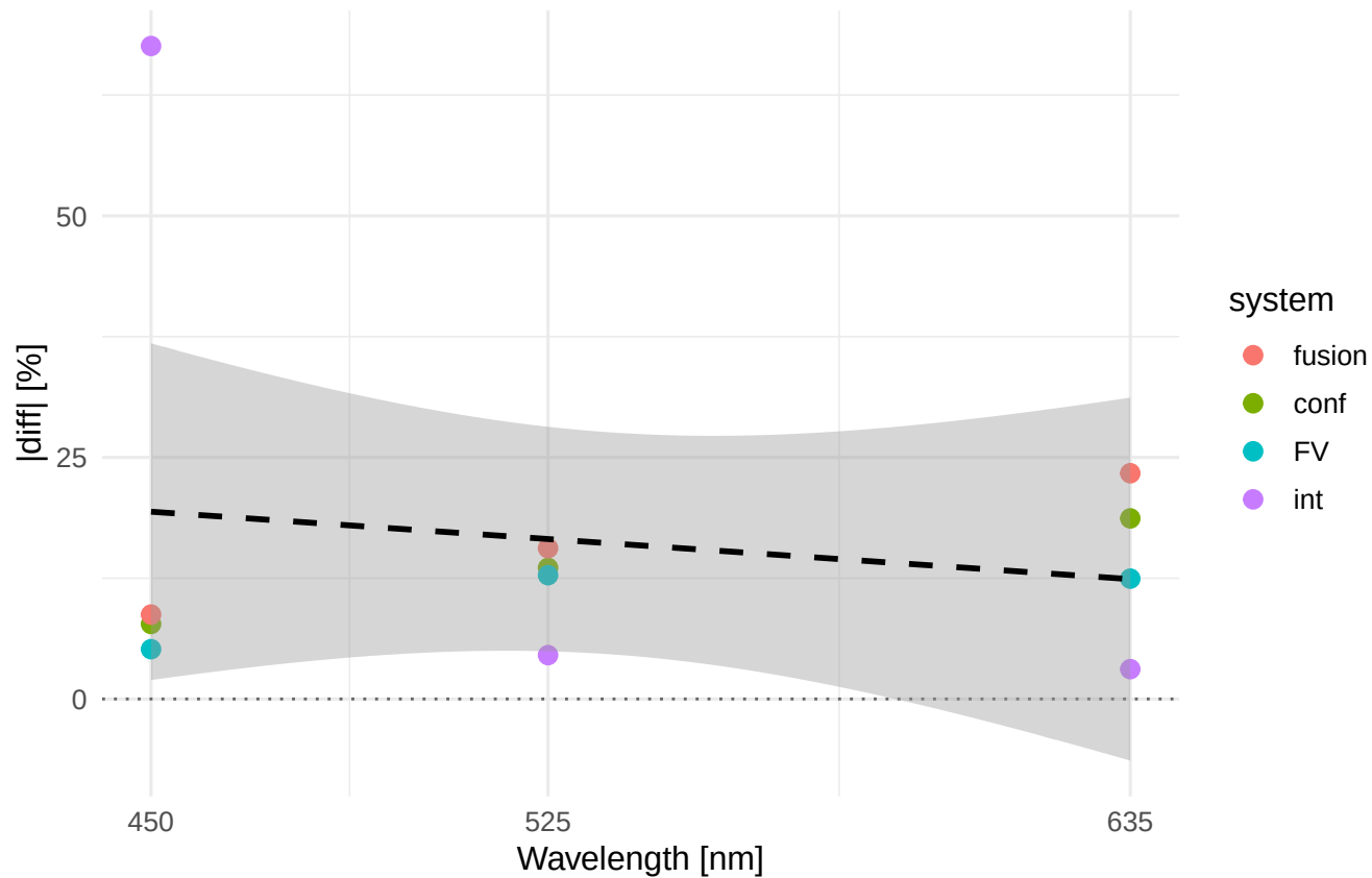
Rq |diff|% vs wavelength Material/process: ELLOR_MR
