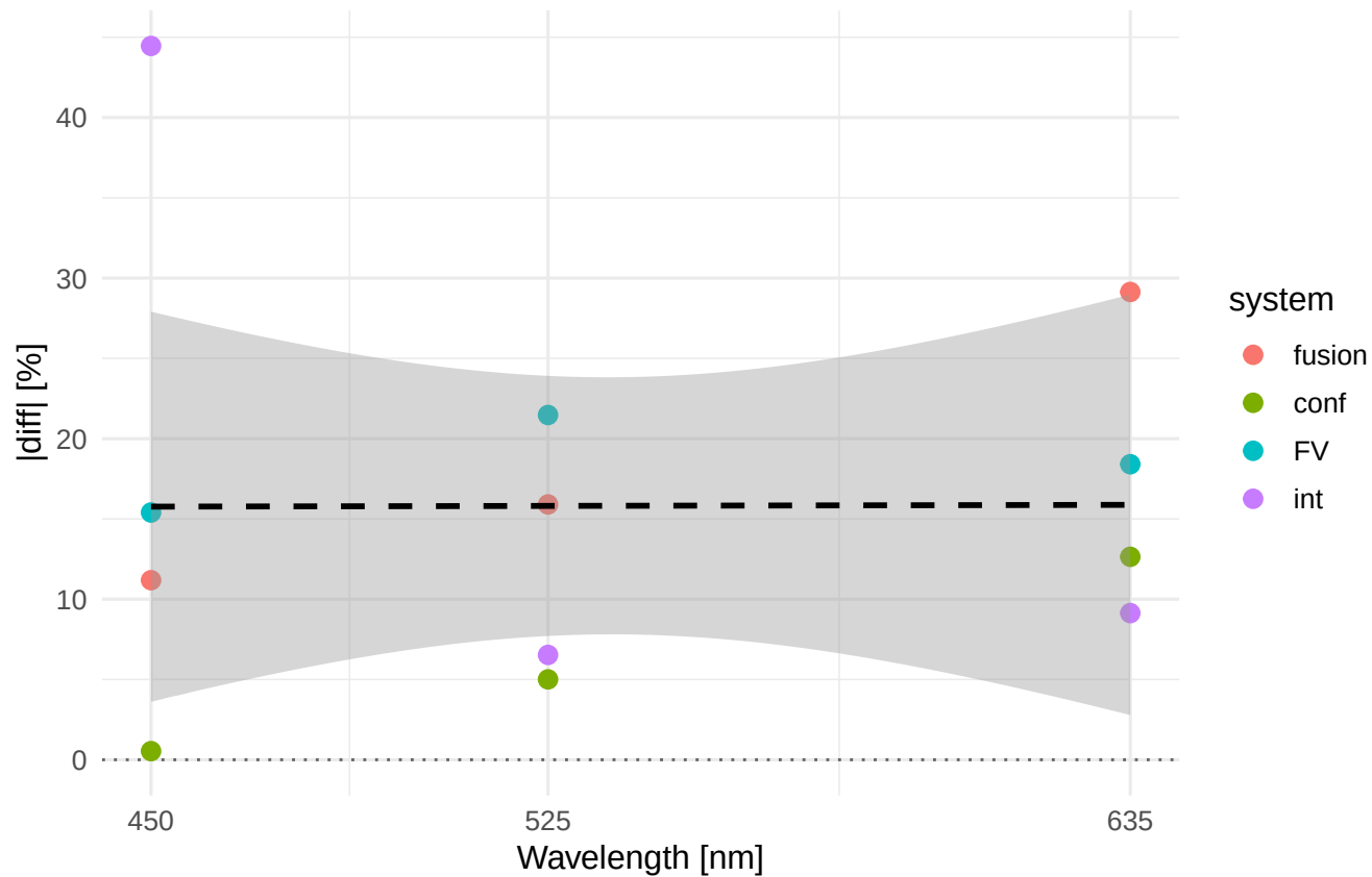
Rq |diff|% vs wavelength Material/process: ELLOR_TF
