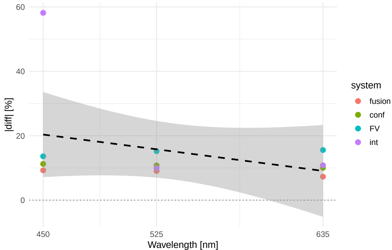
Rq |diff|% vs wavelength Material/process: ELLOR_TR
