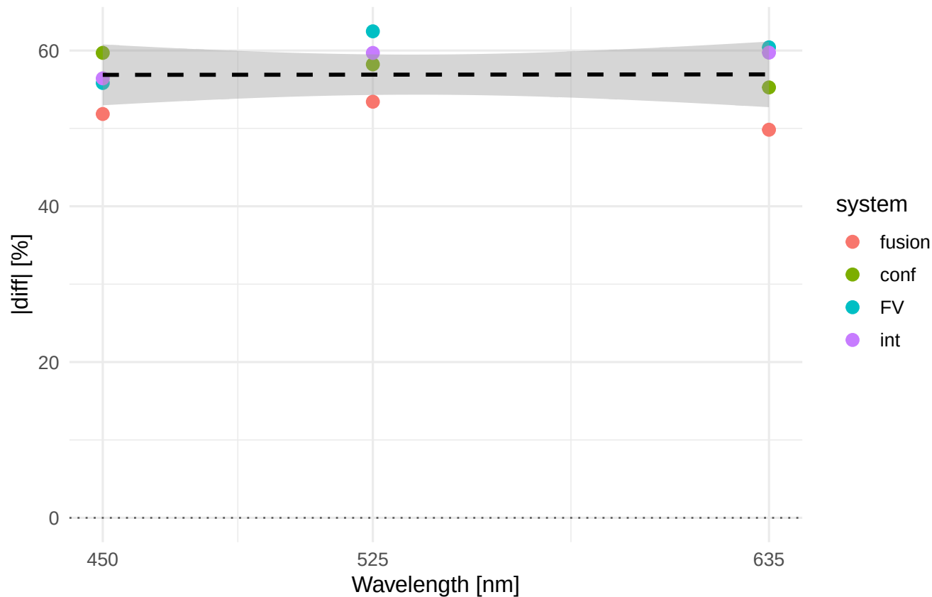
Rq |diff|% vs wavelength Material/process: MO58A_TF
