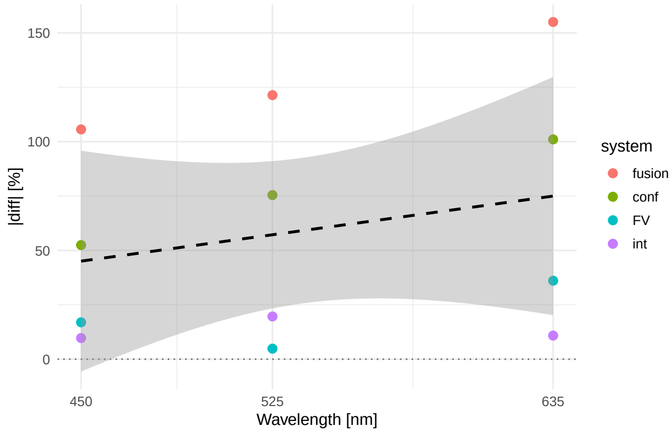
Rq |diff|% vs wavelength Material/process: Ti6Al4V_GLA
