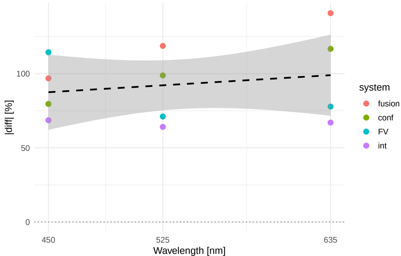
Rq |diff|% vs wavelength Material/process: Ti6Al4V_GRI
