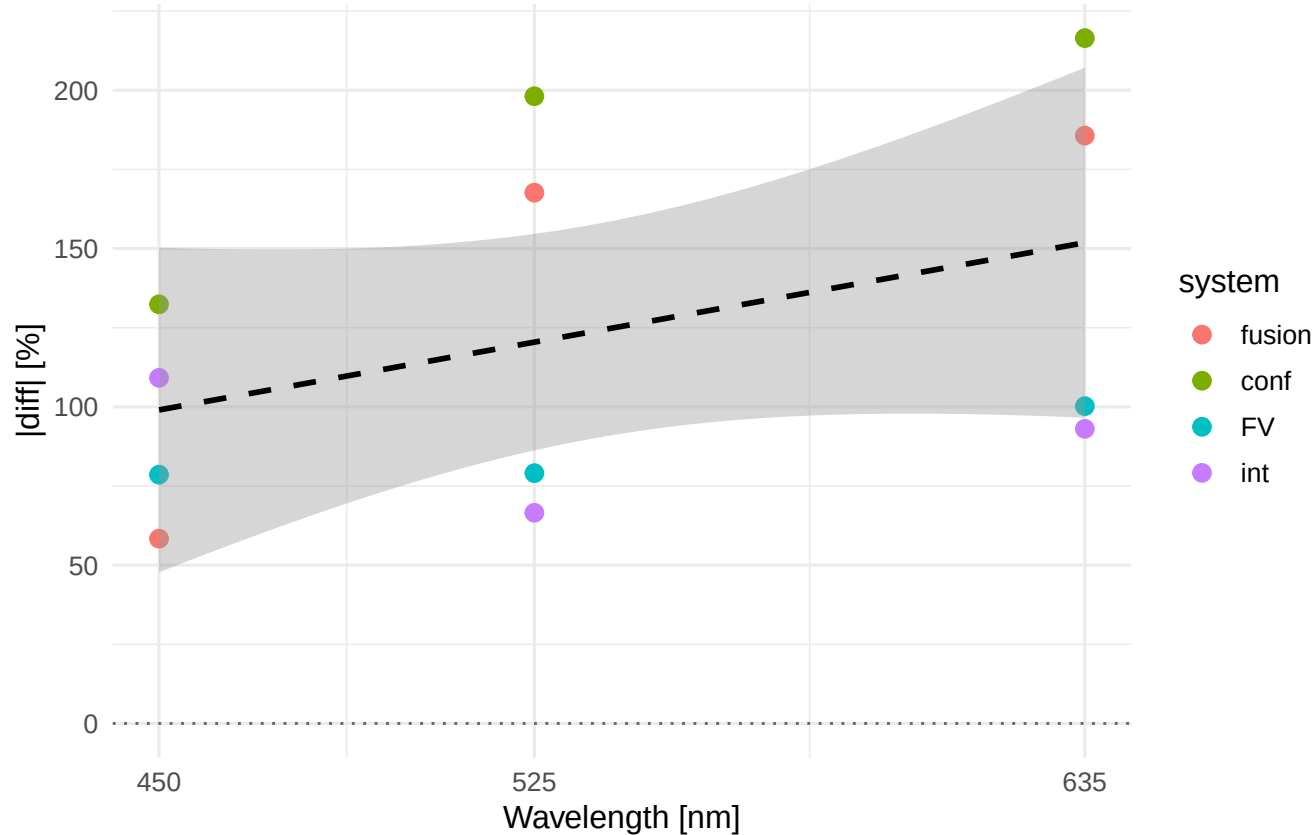
Rsk |diff|% vs wavelength Material/process: 14301_HON
