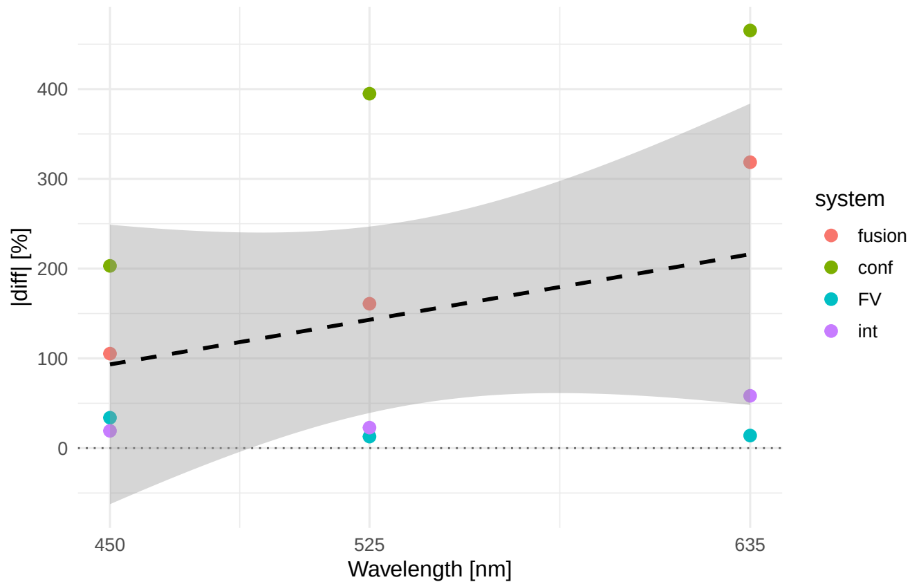
Rsk |diff|% vs wavelength Material/process: Al7075_GLA
