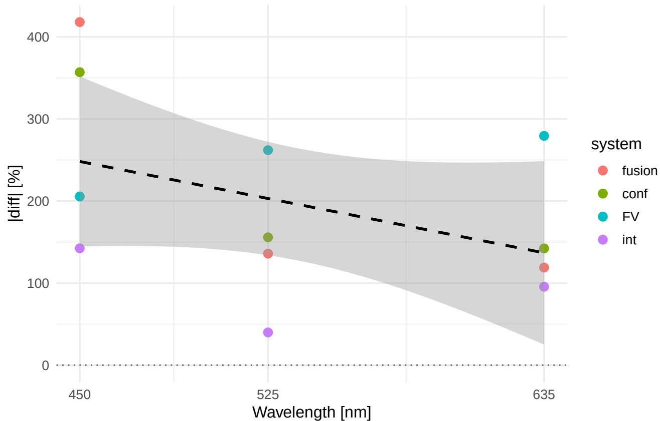
Rsk |diff|% vs wavelength Material/process: Al7075_WEDM_F
