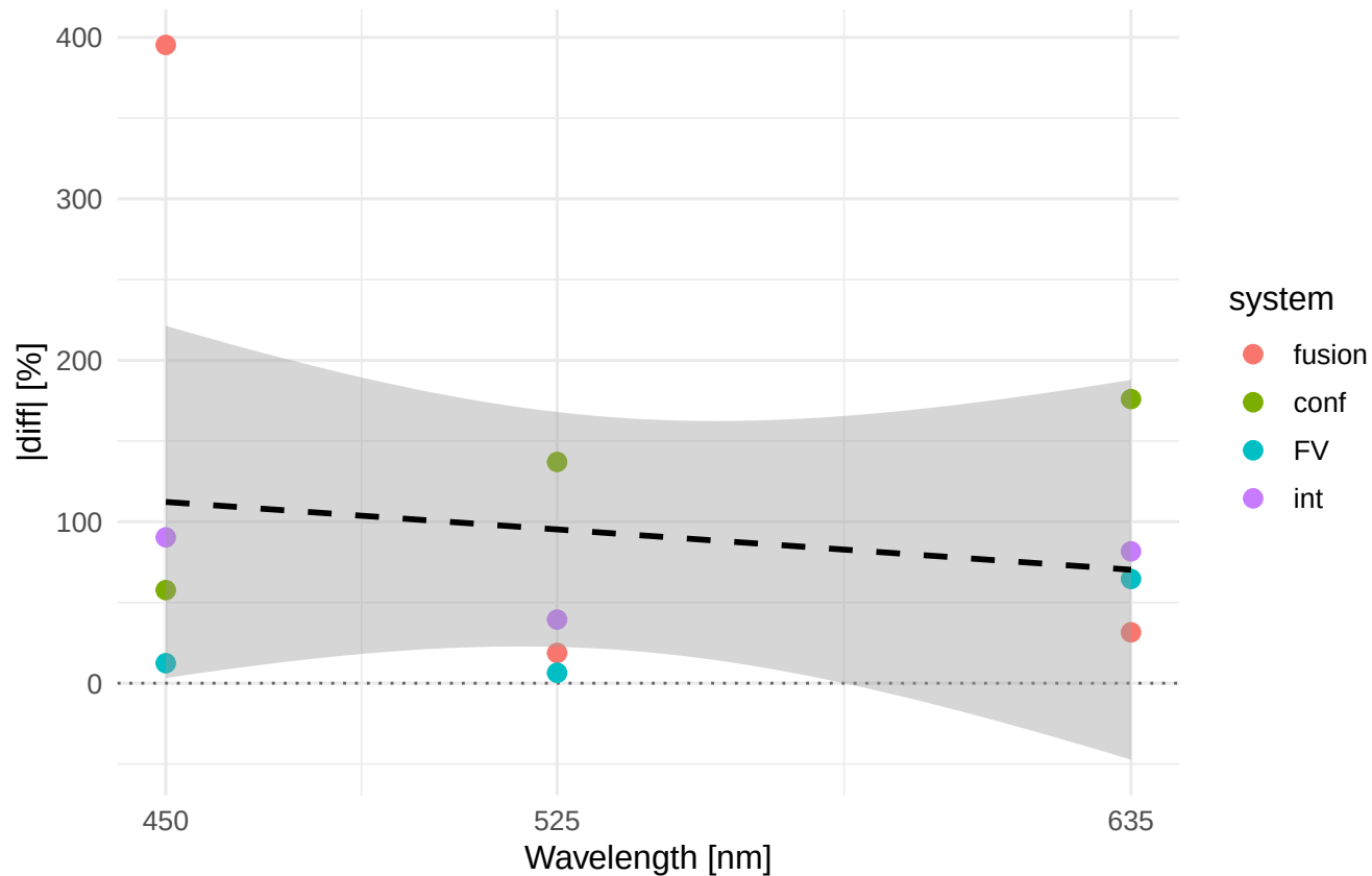
Rsk |diff|% vs wavelength Material/process: C45_WEDM_F
