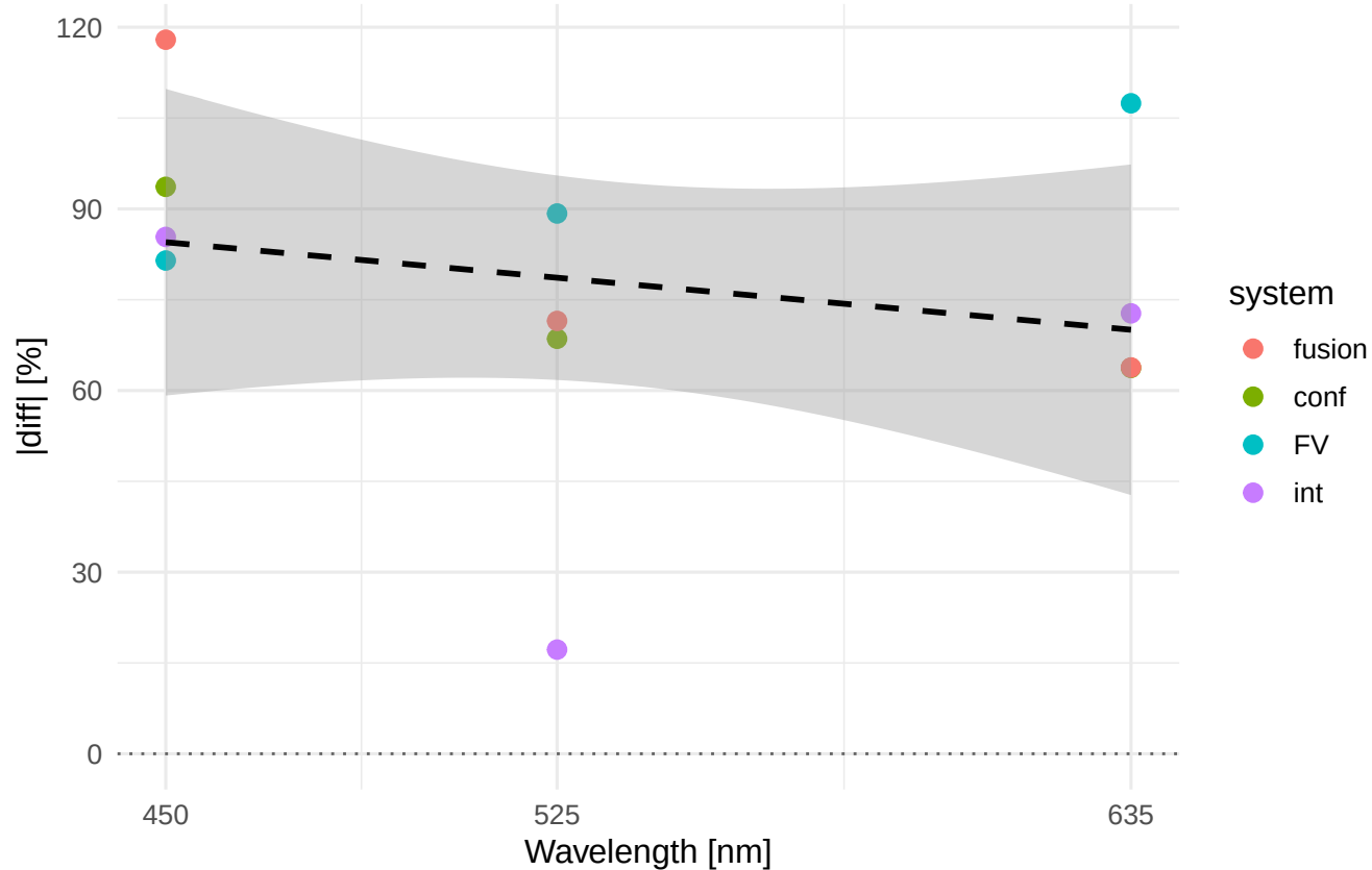
Rsk |diff|% vs wavelength Material/process: ELLOR_HON
