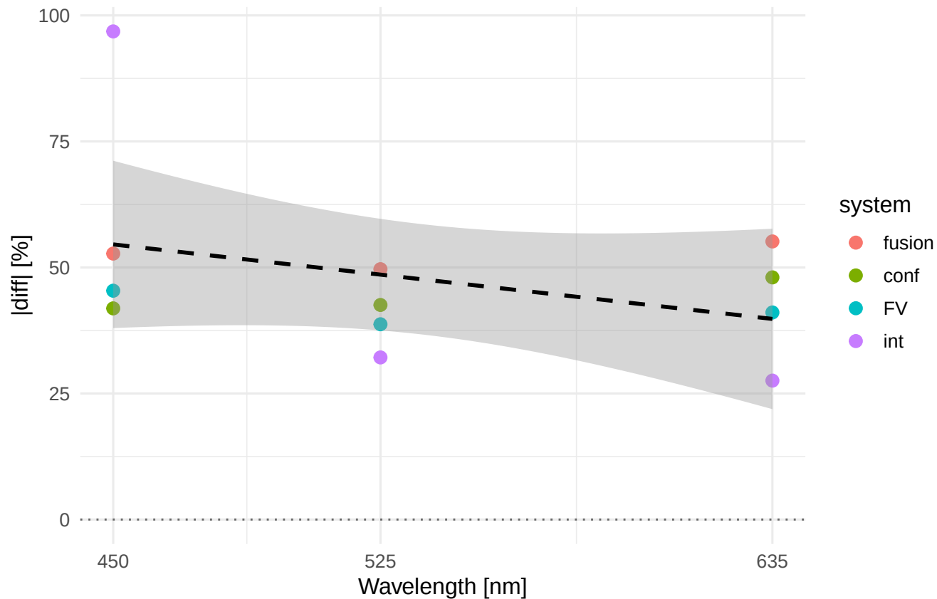
Rsk |diff|% vs wavelength Material/process: ELLOR_WEDM_R
