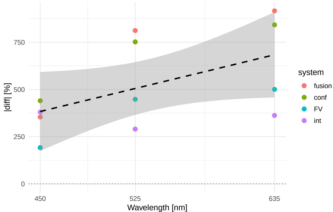
Rsk |diff|% vs wavelength Material/process: MO58A_HON
