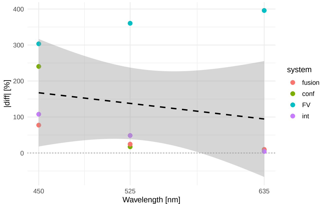
Rsk |diff|% vs wavelength Material/process: MO58A_WEDM_F
