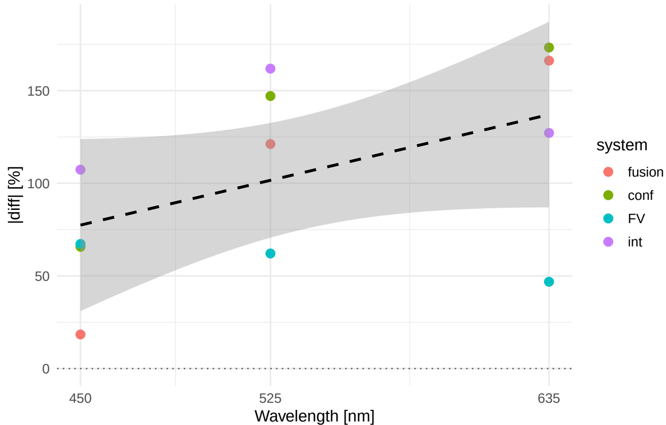
Rsk |diff|% vs wavelength Material/process: Ti6Al4V_GLA
