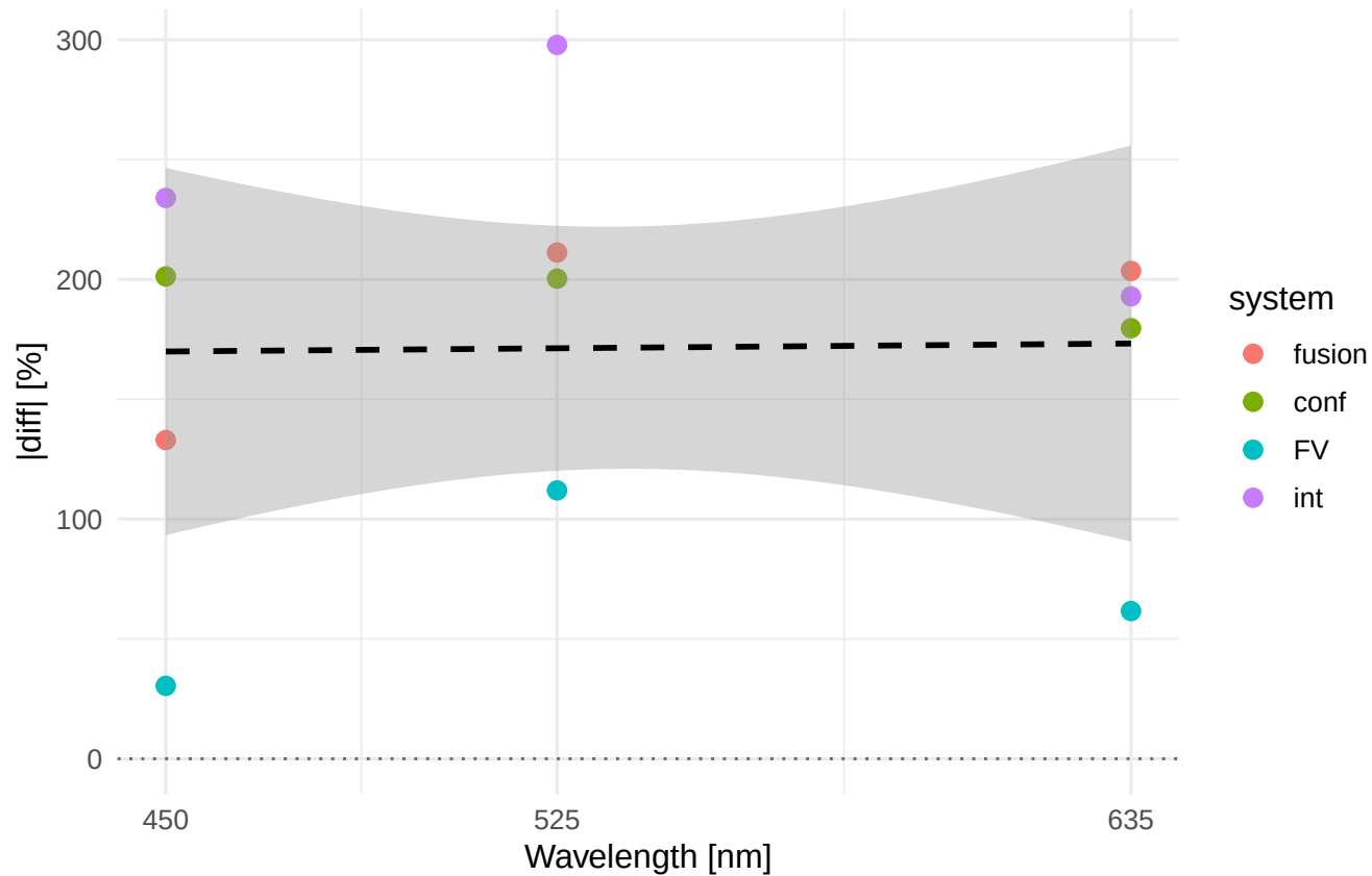
Rsk |diff|% vs wavelength Material/process: Ti6Al4V_GRI
