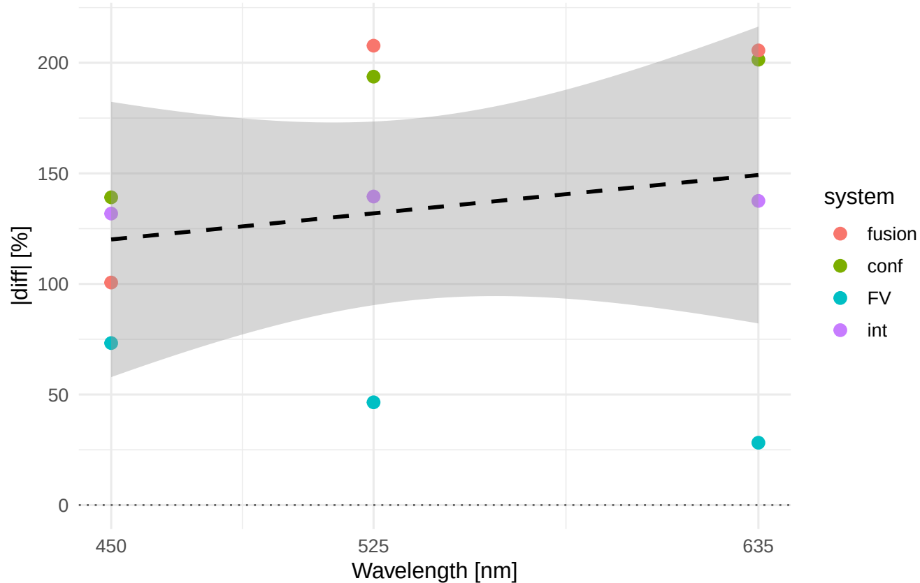
Rsk |diff|% vs wavelength Material/process: Ti6Al4V_HON
