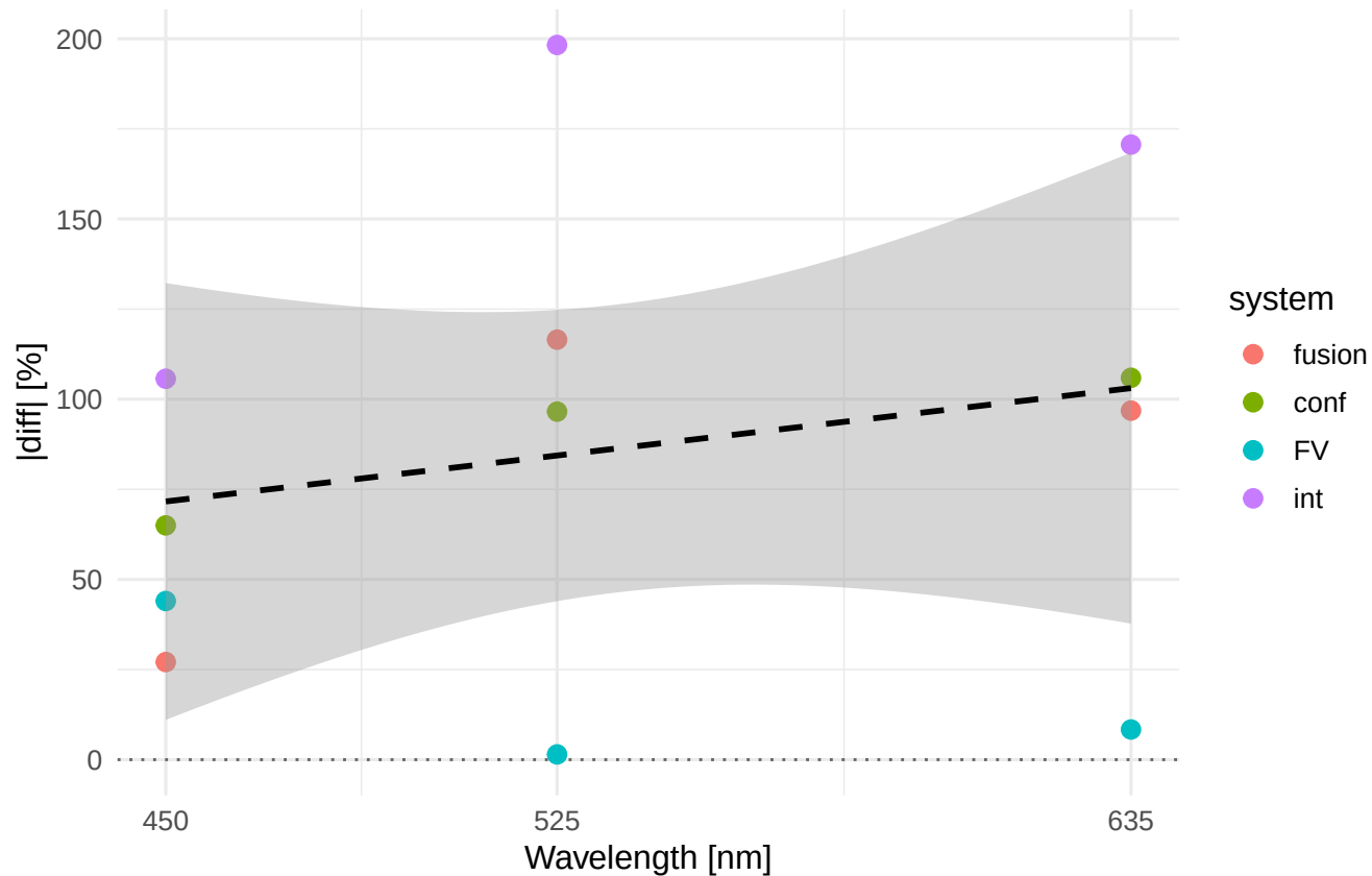
Rsk |diff|% vs wavelength Material/process: Ti6Al4V_WEDM_F
