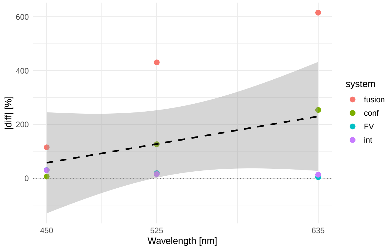
Rsk |diff|% vs wavelength Material/process: Ti6Al4V_WEDM_R
