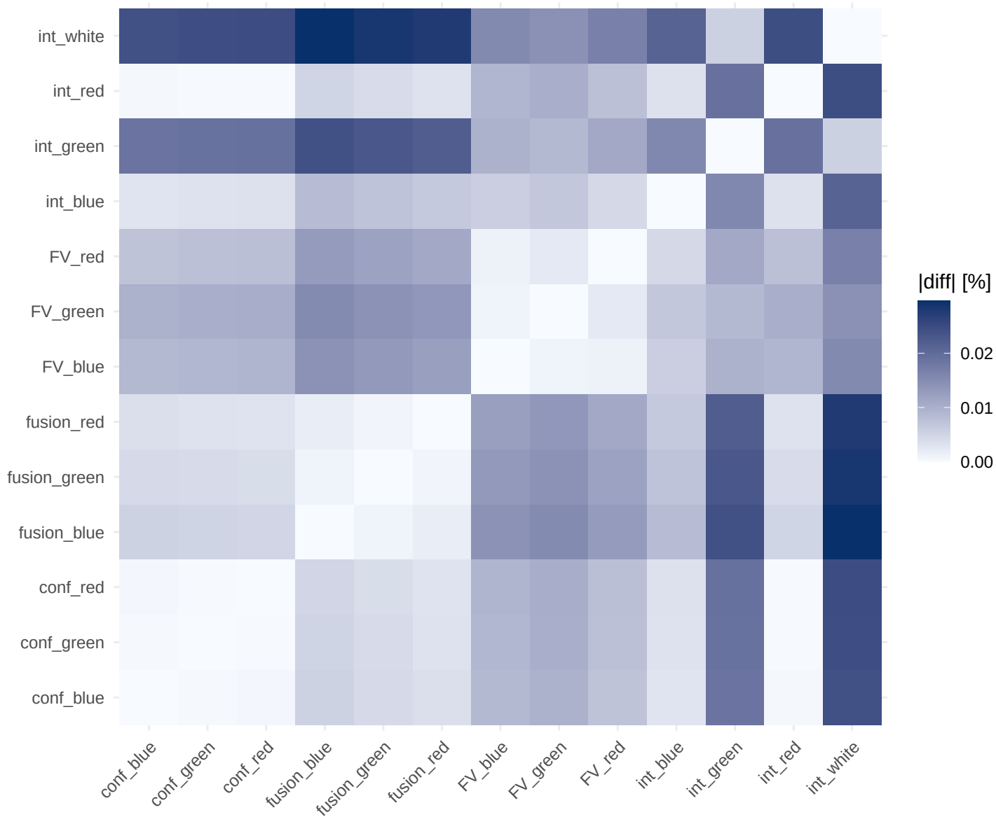
Rsm technique distance heatmap ( |\text{diff}| \% )
