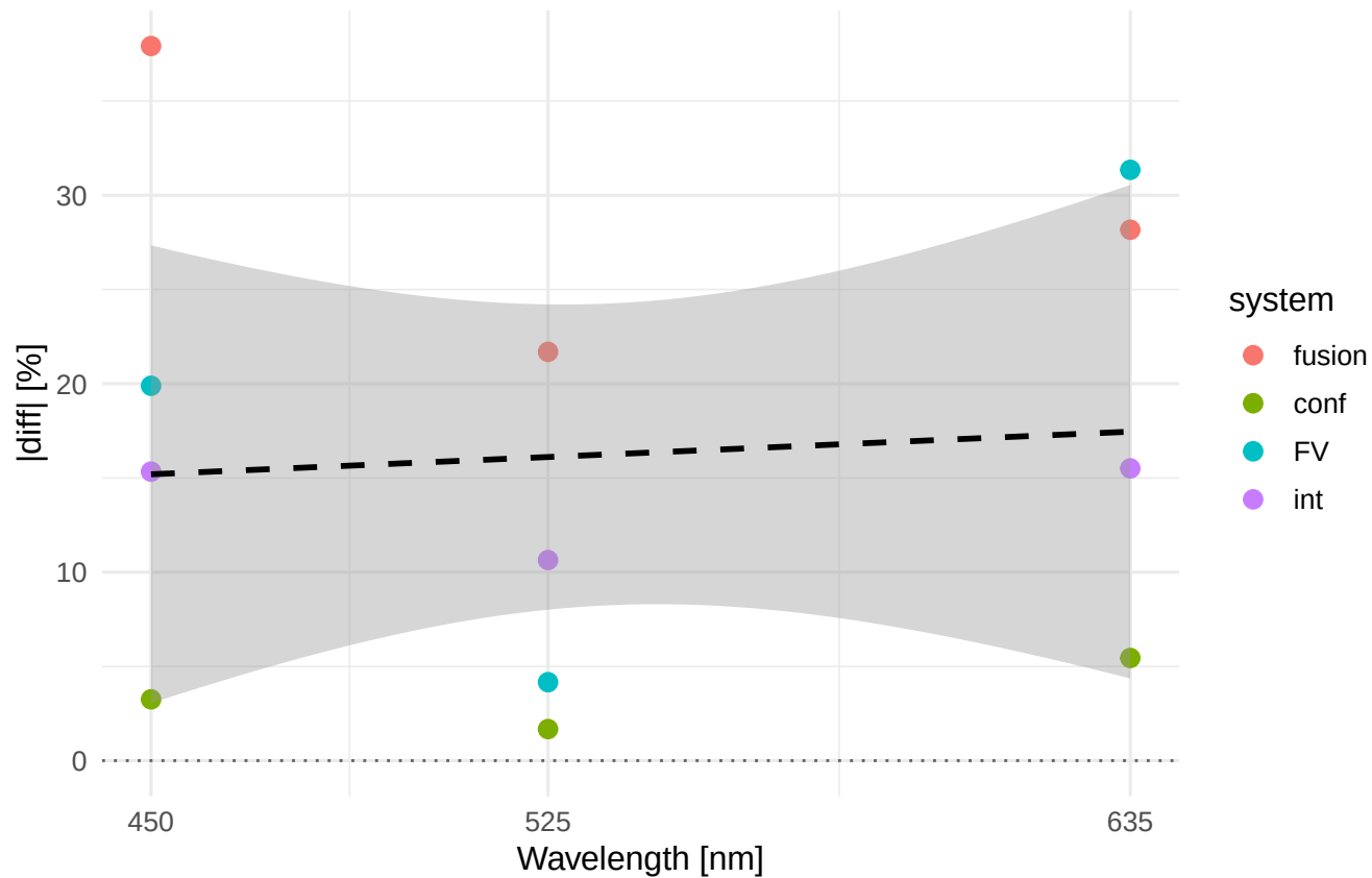
Rt |diff|% vs wavelength Material/process: 14301_GRI
