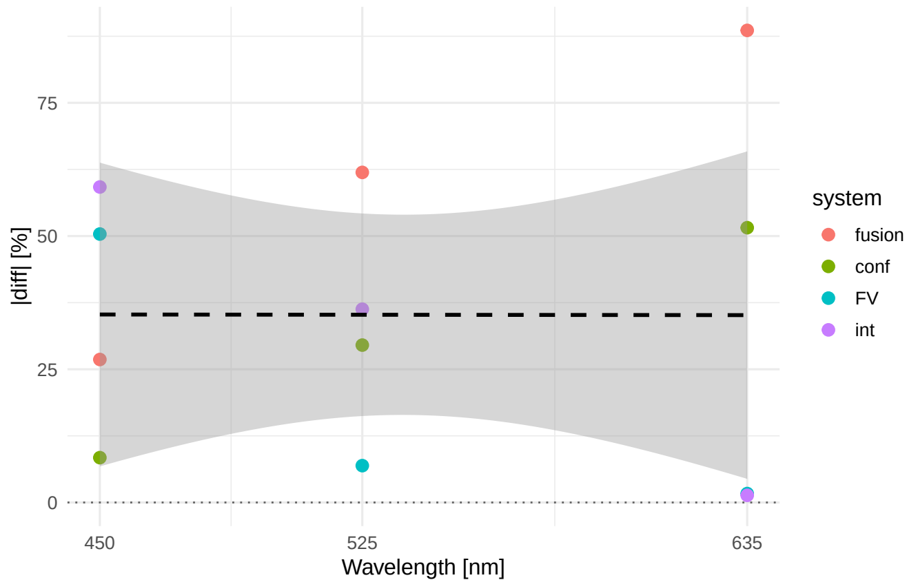
Rt |diff|% vs wavelength Material/process: 14301_MF
