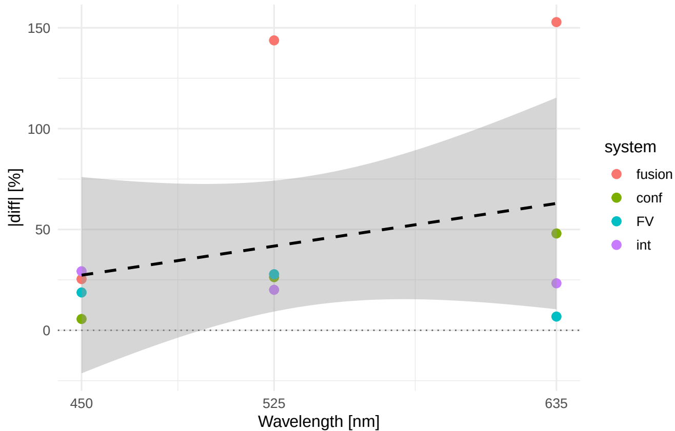
Rt |diff|% vs wavelength Material/process: Al7075_GLA
