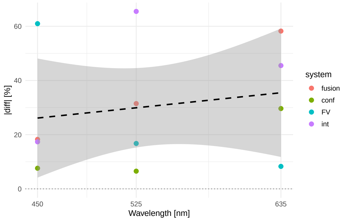
Rt |diff|% vs wavelength Material/process: Al7075_MF
