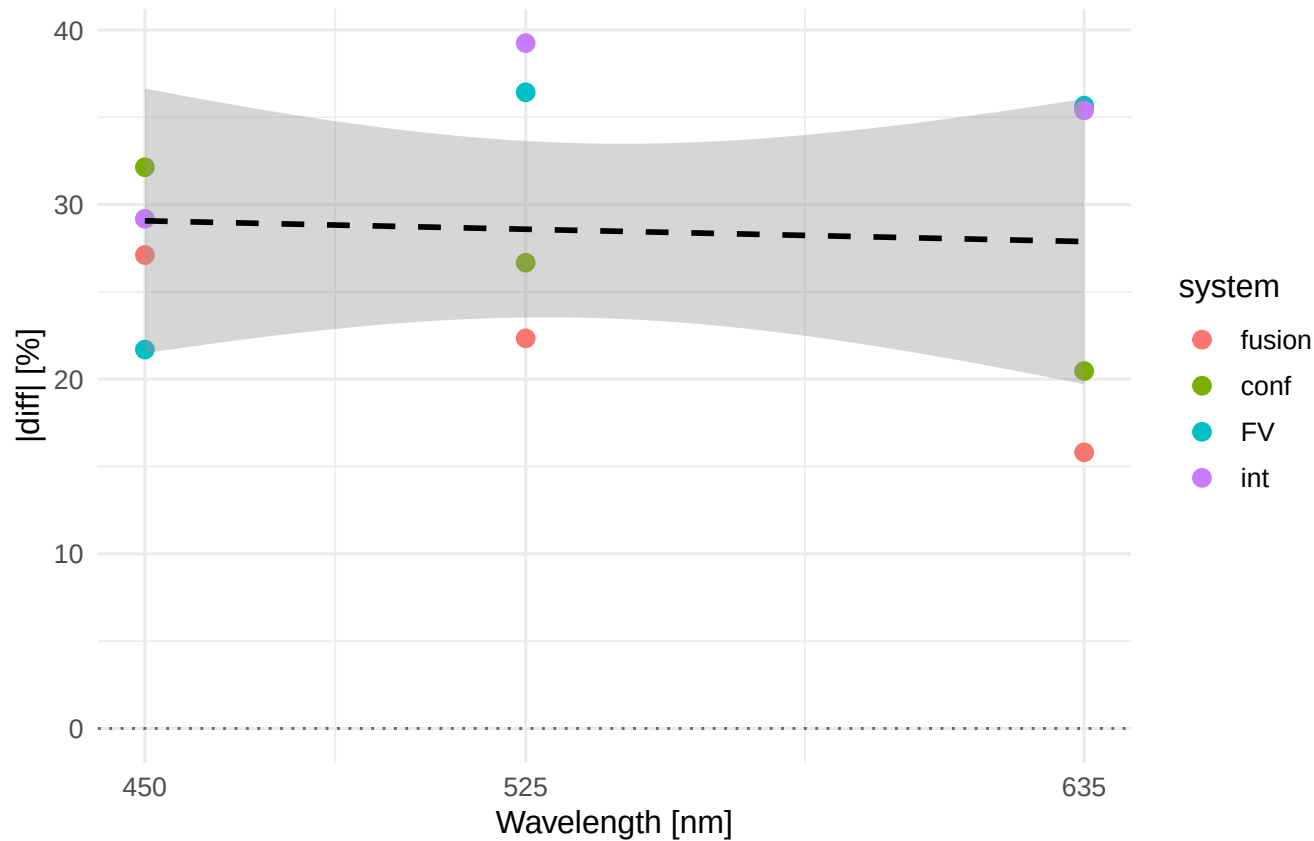
Rt |diff|% vs wavelength Material/process: Al7075_TR
