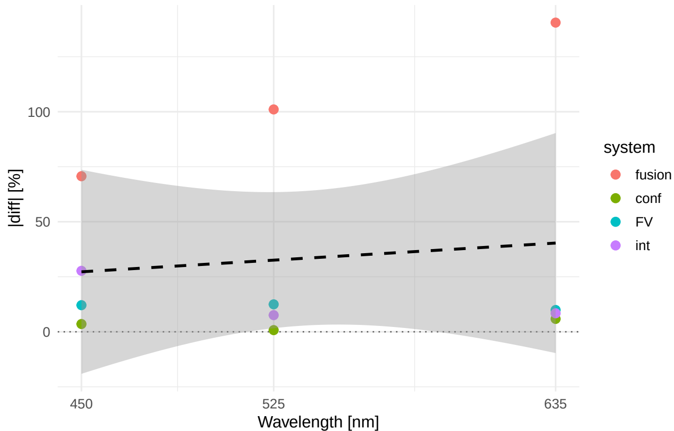
Rt |diff|% vs wavelength Material/process: C45_WEDM_R
