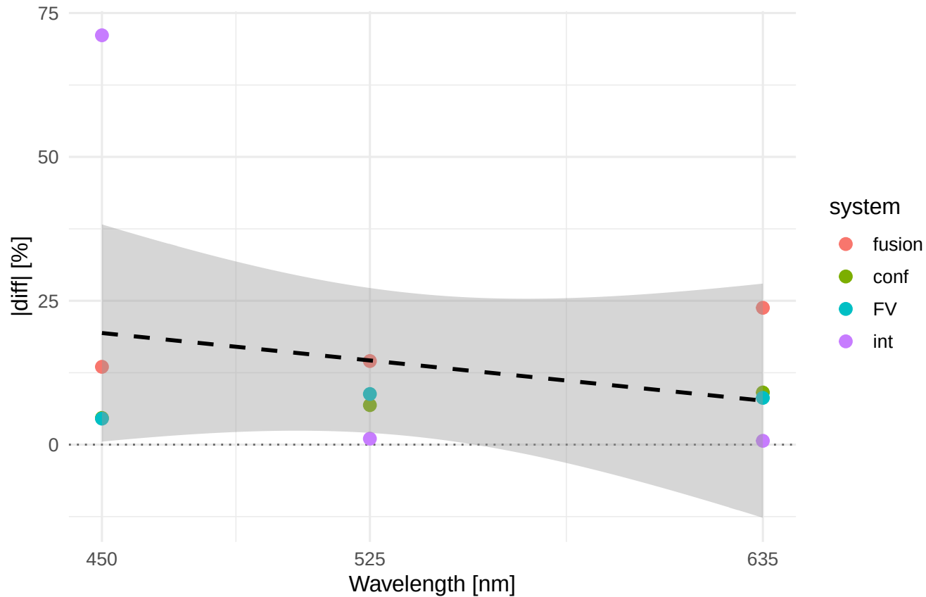
Rt |diff|% vs wavelength Material/process: ELLOR_MR
