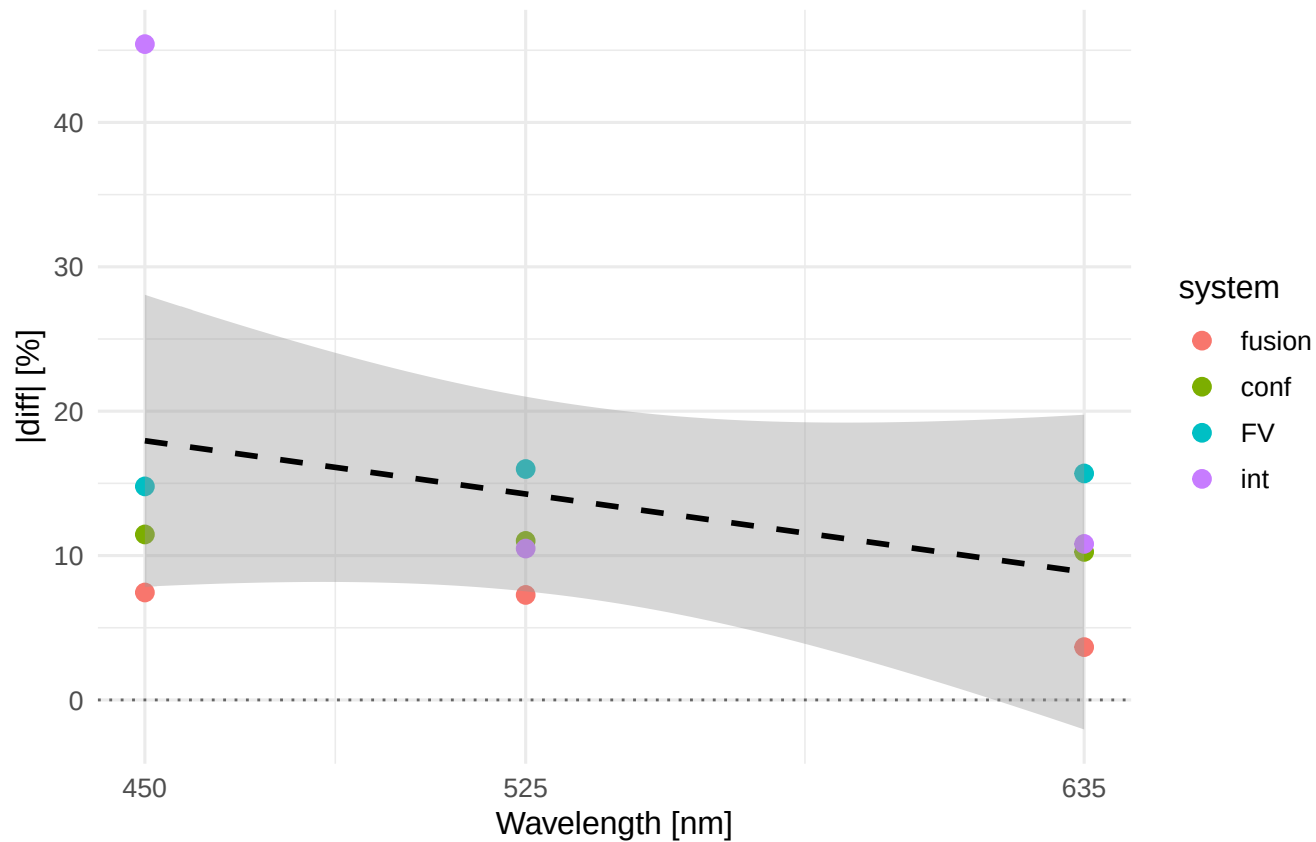
Rt |diff|% vs wavelength Material/process: ELLOR_TR
