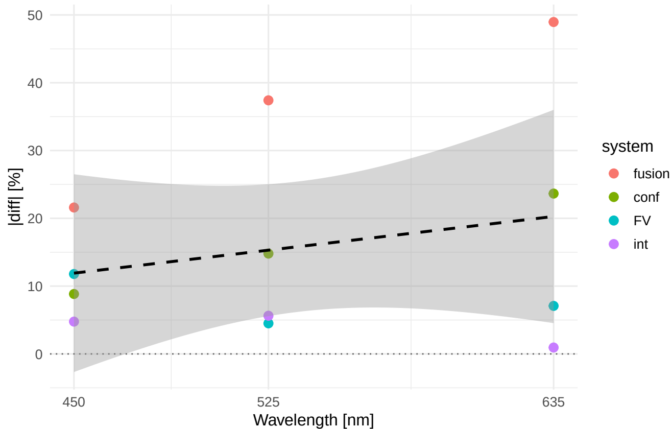
Rv |diff|% vs wavelength Material/process: 14301_GRI
