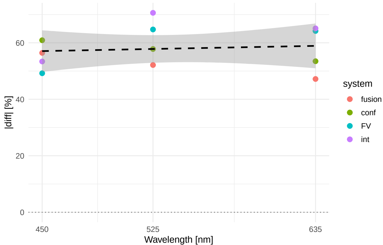
Rv |diff|% vs wavelength Material/process: Al7075_TR
