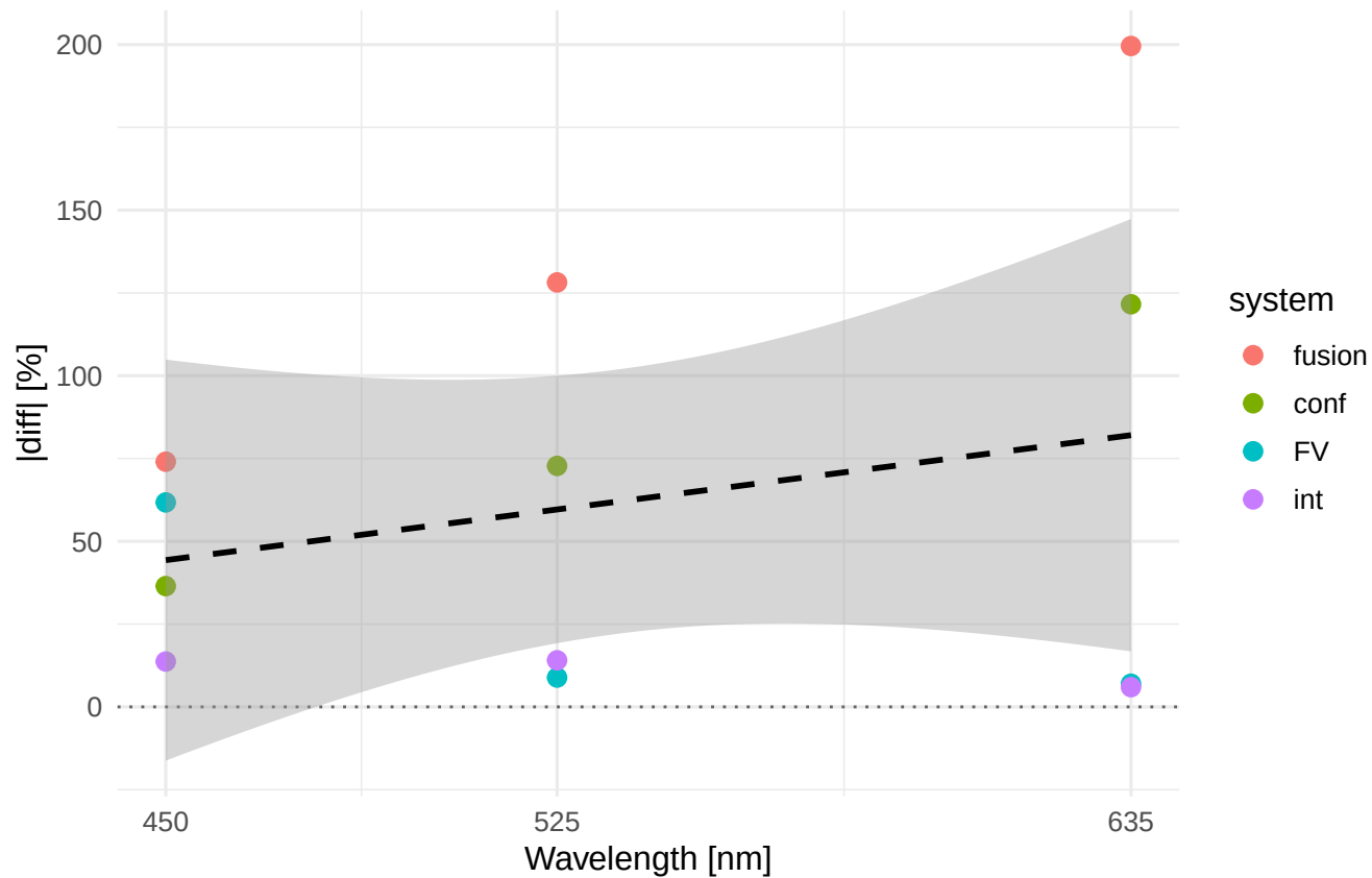
Rv |diff|% vs wavelength Material/process: ELLOR_HON
