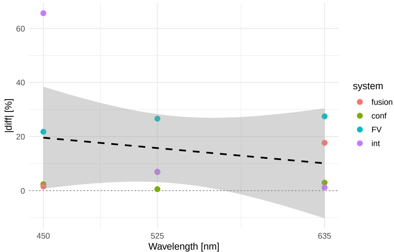
Rv |diff|% vs wavelength Material/process: ELLOR_TF
