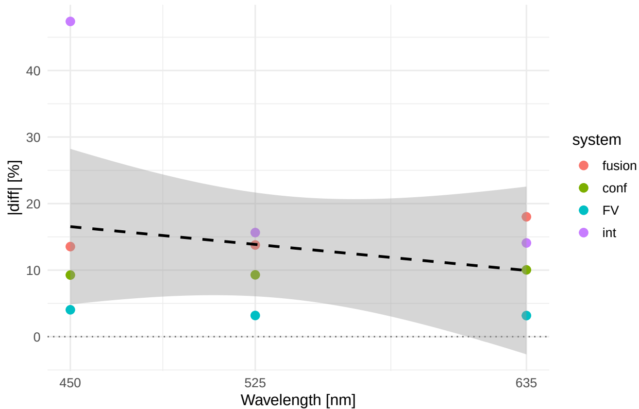
Rv |diff|% vs wavelength Material/process: ELLOR_TR
