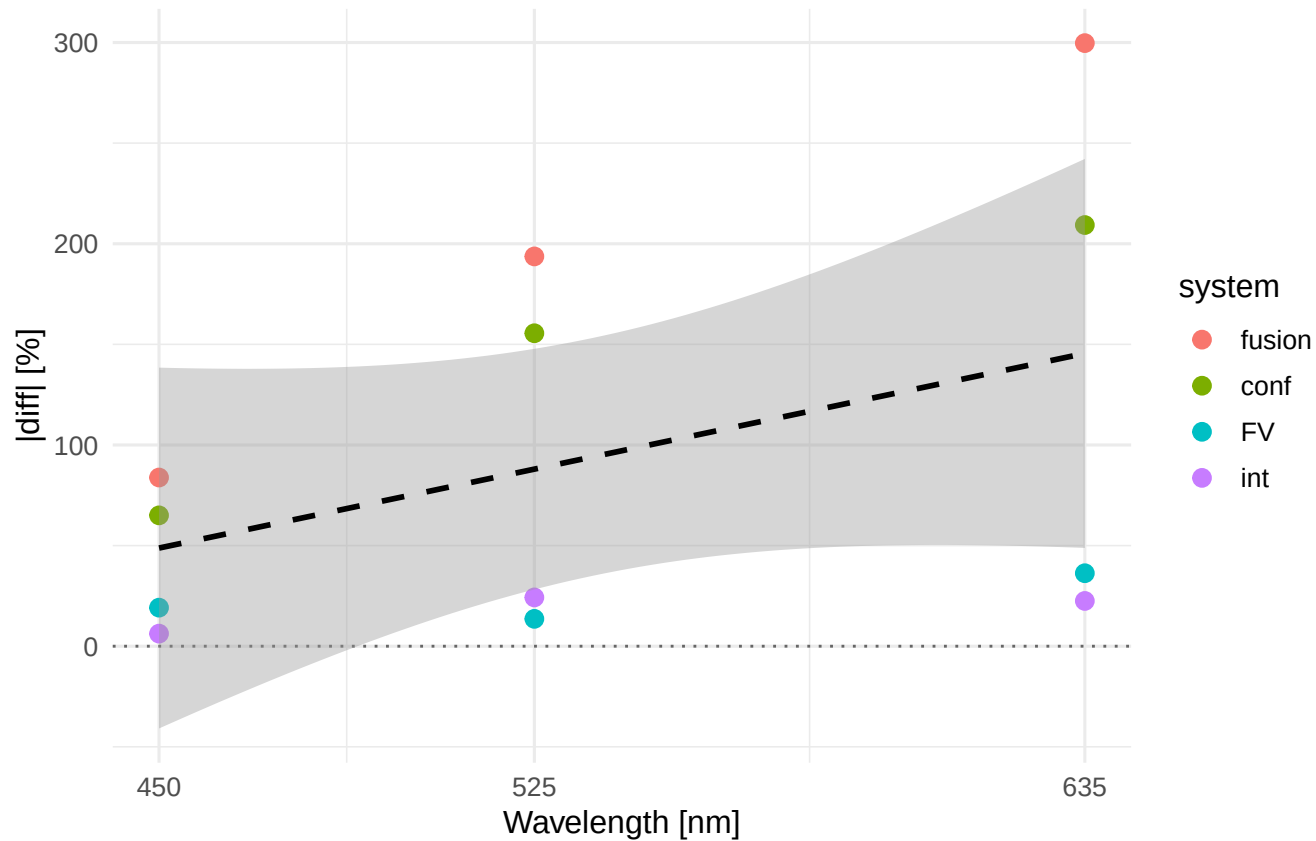
Rv |diff|% vs wavelength Material/process: MO58A_GLA
