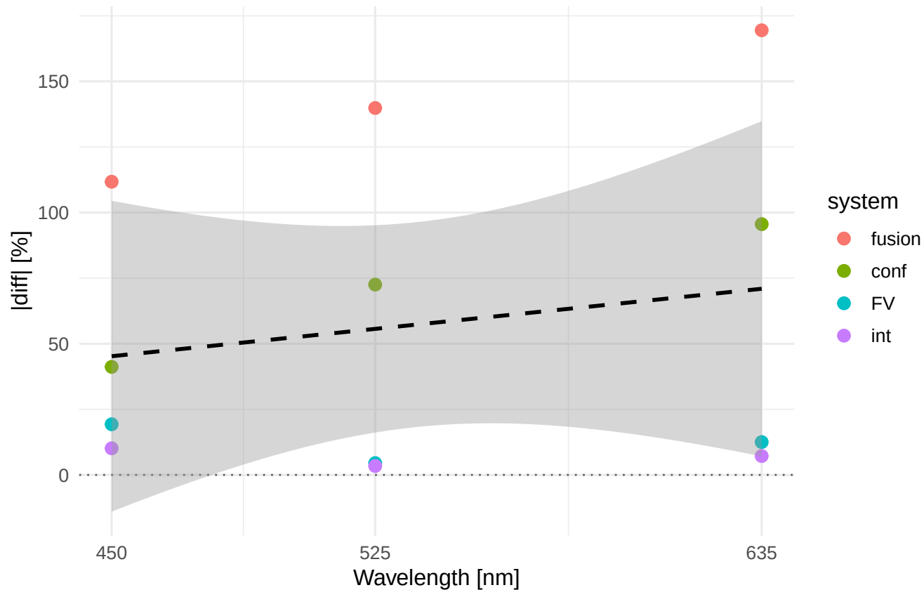
Rv |diff|% vs wavelength Material/process: MO58A_WEDM_F
