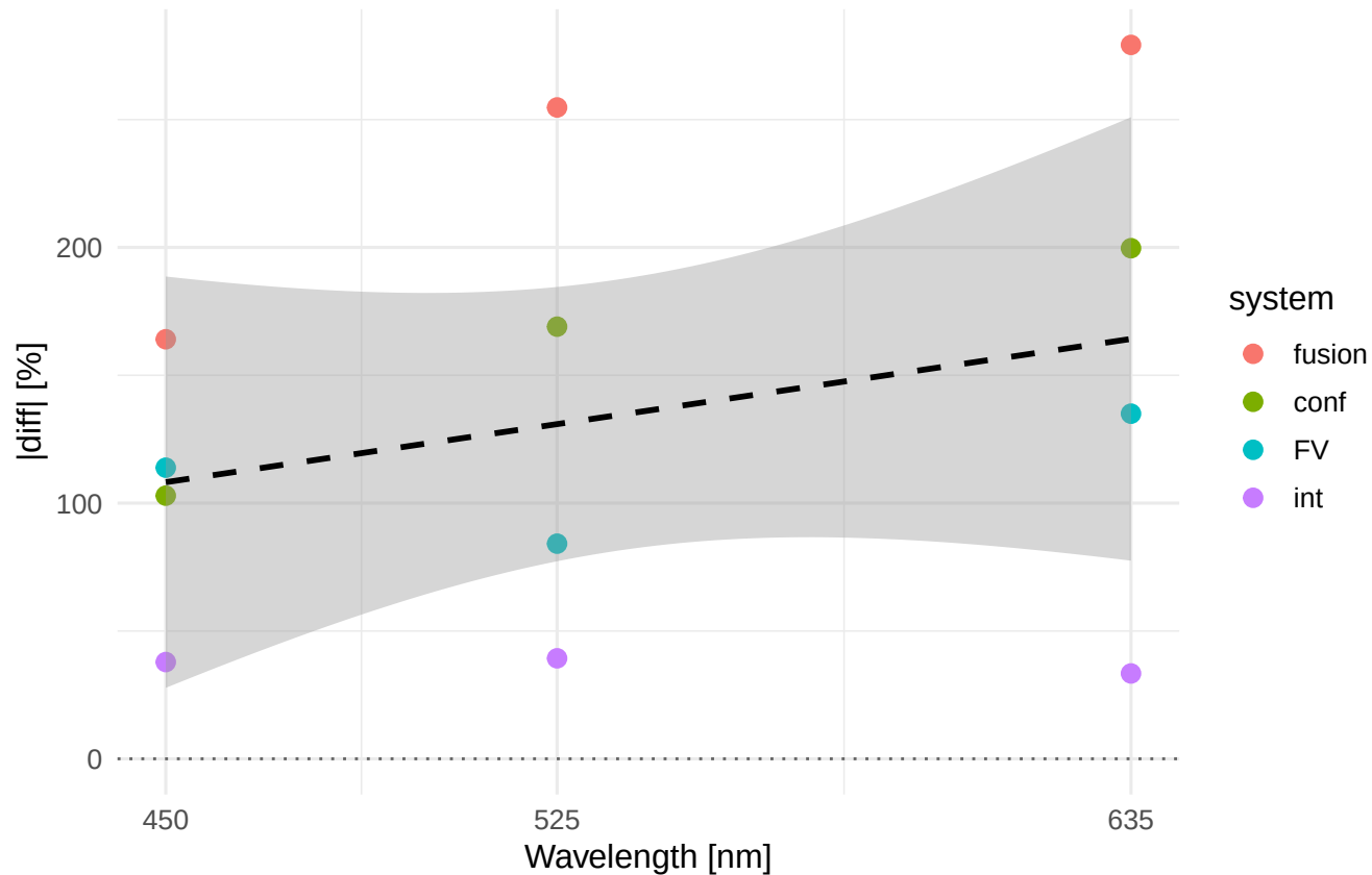
Rv |diff|% vs wavelength Material/process: Ti6Al4V_HON
