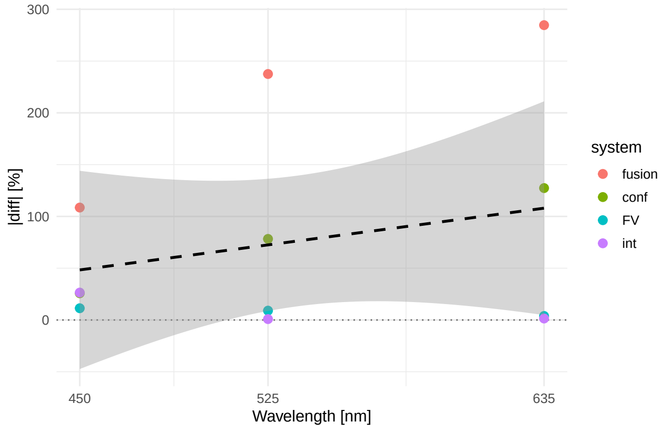
Rv |diff|% vs wavelength Material/process: Ti6Al4V_WEDM_R
